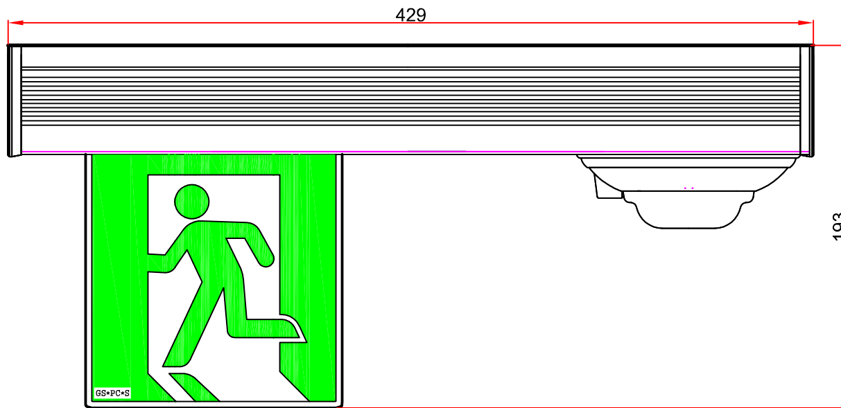
FRONT VIEW
