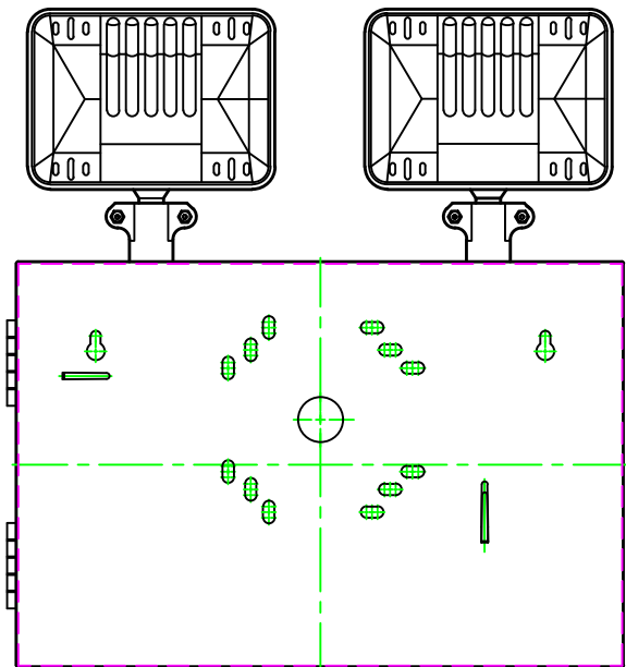
REAR VIEW
