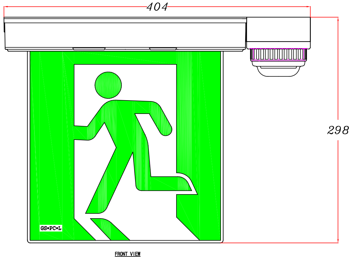
FRONT VIEW
